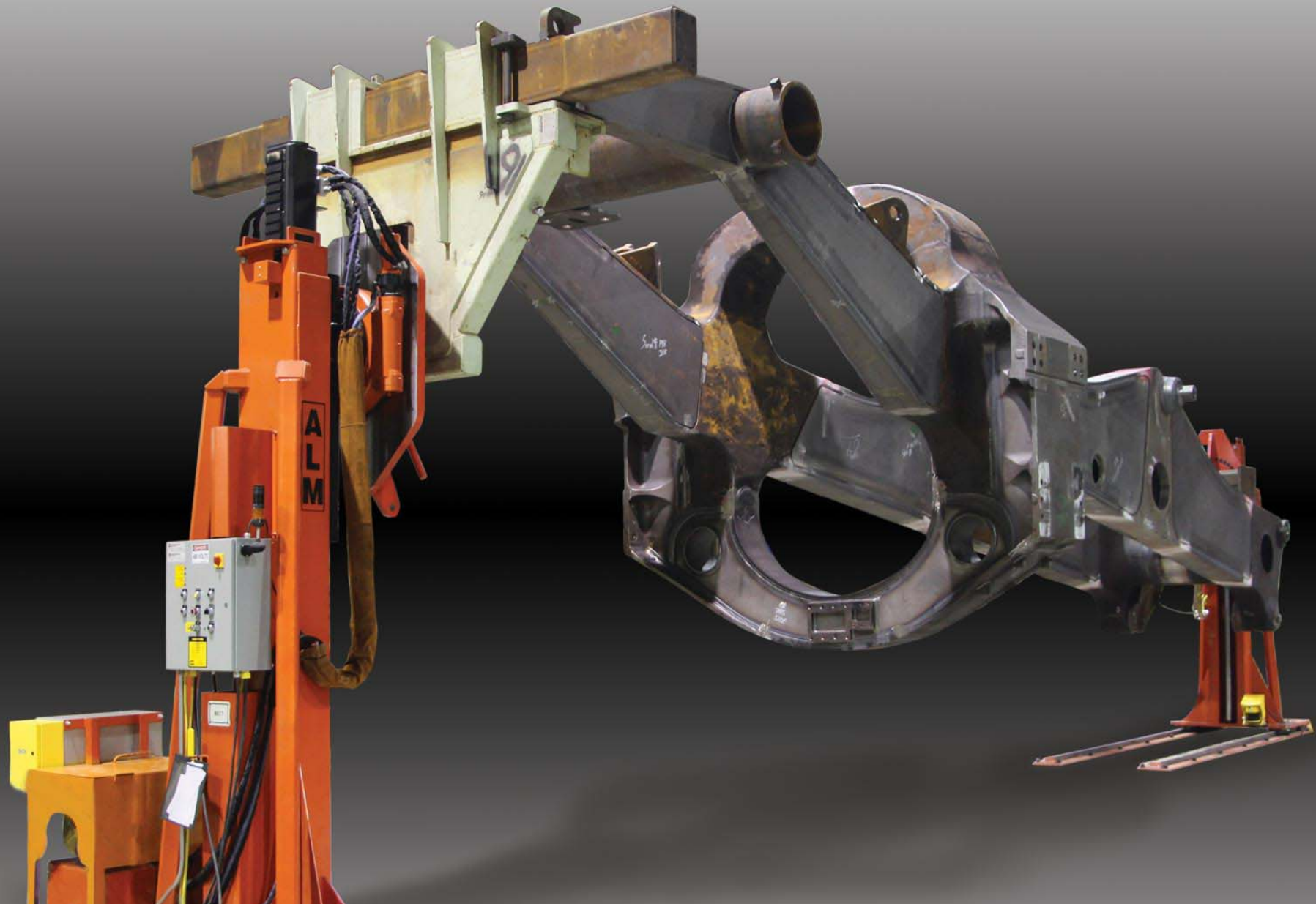
MHL-2P 75,000 lb. Capacity with 73 inches of verticle lift.
